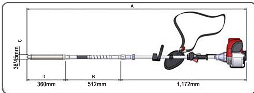
HOPPT® Hand-Held Portable Concrete Vibrator with Padded Shoulder-Harness
